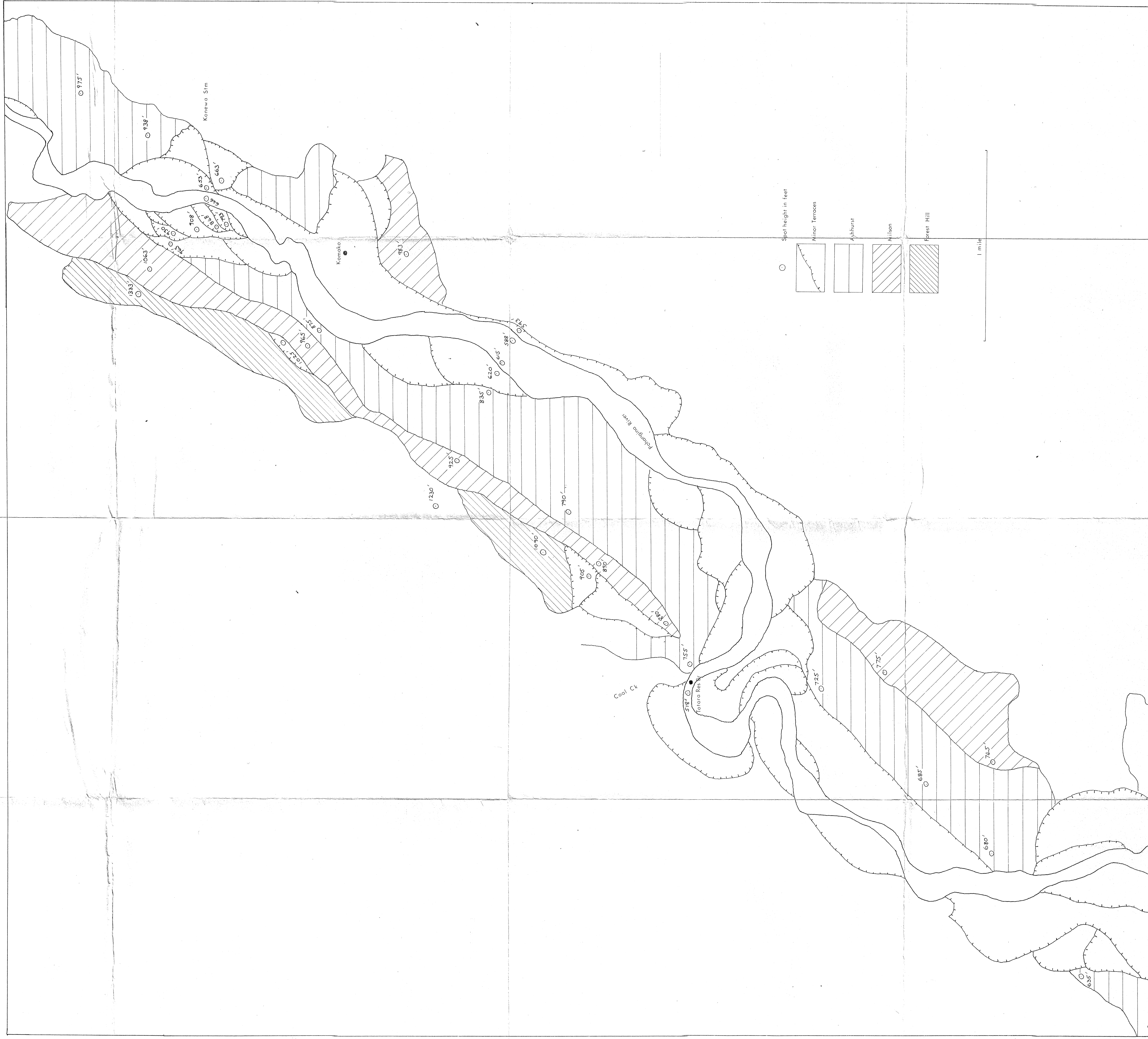
River terraces between Ohinetapu Stream and Konewa Stream
