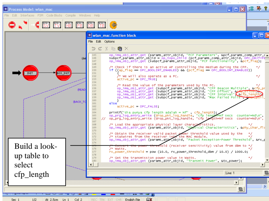
Figure B-1(b) Showing the Calling Function in OPNET to Create the MDSS Look-up Table
