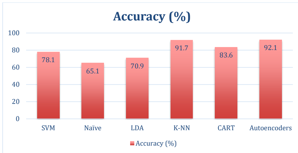
Figure 8: The accuracy results of different algorithms
