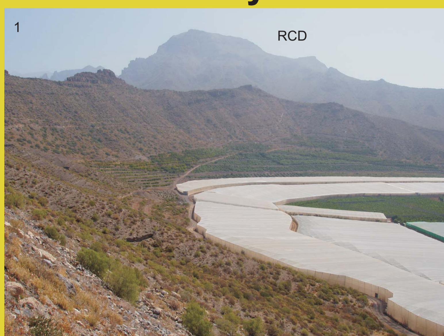
Maar crater of the Caldera del Rey from the west. In the background the Roque del Conde Massif (RCD) blocks are visible.
