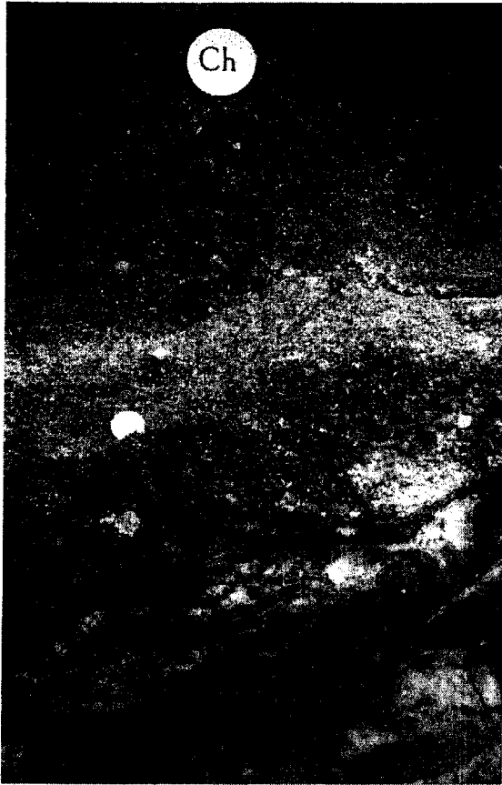
Fig. 12. Small chutes and scours (Ch and arrows with dashed lines) on the lower bed surface of a coarse grained bed (Lithofacies 1) from the Kiserdõ-tetõ (Tihany) outcrop. Their elongation is identical with the bed dip direction. The coin is 2.5 cm in diameter.
