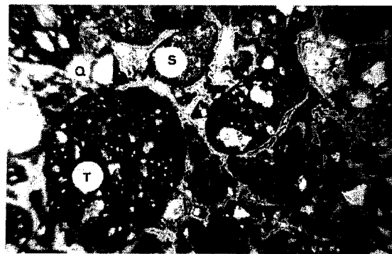
Fig. 14. Reworked tuff from fine-grained lithofacies (L2, Kiserdö-tető, Tihany) in thin section. Note the roundness of the grains as well as their dark colour rim (mostly altered glass). S, sideromelane; T, tachylite, Q, quartz. The shorter side of the picture is 4 mm.
