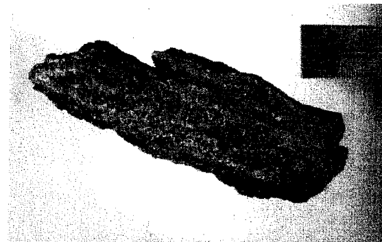
Fig. 11. Hand specimen of a coarse-grained, grain-supported lapilli tuff from Csúcs-hegy (Tihany).
