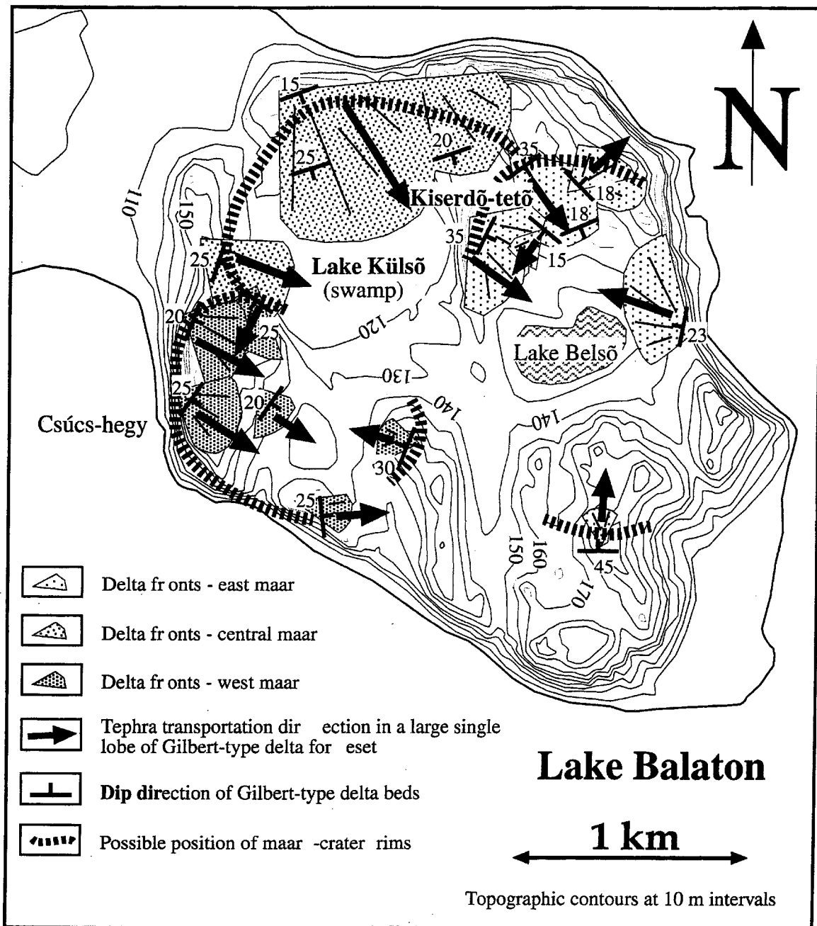
Fig. 3. Reconstruction of large Gilbert-type delta fronts on the Tihany peninsula. Different patterns represent different lobes of large Gilbert-type delta fronts. Delta fronts with similar pattern belong to the same maar crater.
