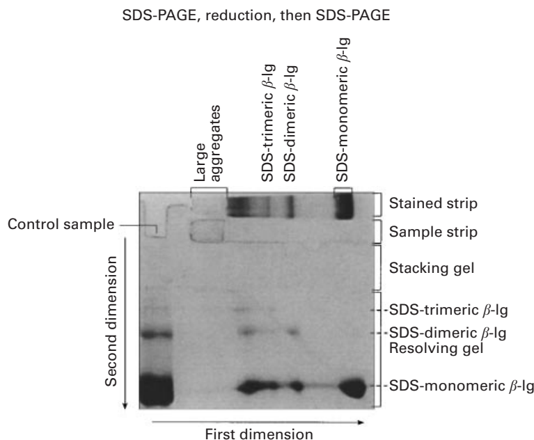
Fig. 2. Two-dimensional electrophoretic patterns of a heat-treated (75 °C for 8 min) solution of \beta -lactoglobulin (100 g/kg solution) in permeate prepared from a solution of whey protein concentrate powder in water (100 g/kg). First dimension, SDS-PAGE without treatment with 2-mercaptoethanol; second dimension, SDS-PAGE of samples within a gel strip that was treated with 2-mercaptoethanol. At the top of each gel a stained gel strip shows the protein bands from the first dimension separation running from left to right. Immediately below this strip is a second strip, which had contained the same protein bands that were used as samples for the second-dimension separation. On the left-hand side, a portion of the corresponding sample was run from top to bottom, to help identify the protein bands.
